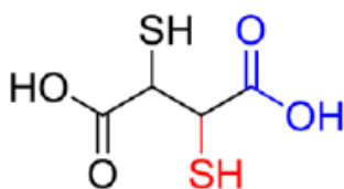
Meso-2,3- dimercaptosuccinic acid
